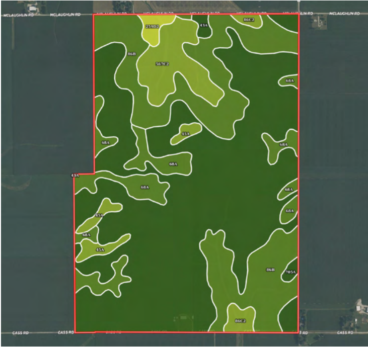
Soil Map
